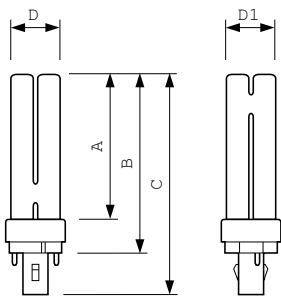
PL-C 18W/865/2P
